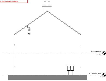
SIDE ELEVATION
